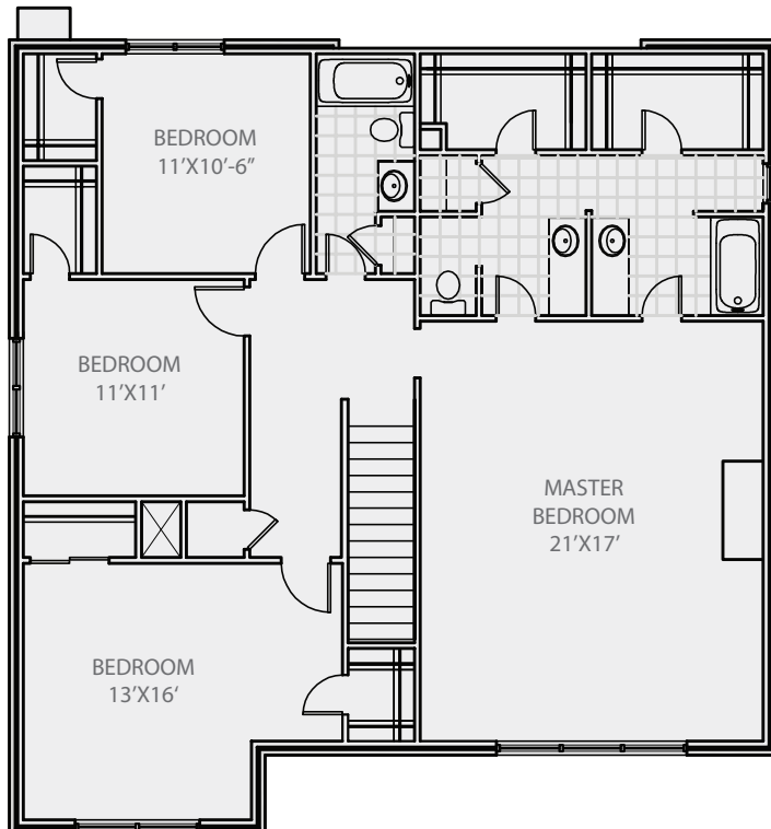
SECOND FLOOR PLAN SCALE: 3/32"=1'-0"
