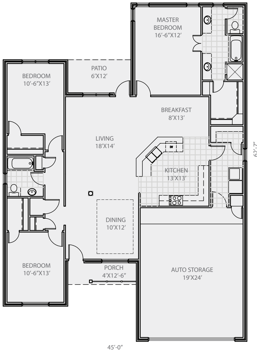
FLOOR PLAN
